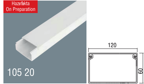
120x60 PVC Kablo Kanalı Kapaklı Satılır Ambalaj: 16m / 8 Boy 120x60 PVC Cable Trunking Complete with cover Packaging: 16m / 8 Pcs
