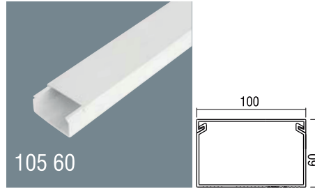
100x60 PVC Kablo Kanalı Kapaklı Satılır Ambalaj: 16m / 8 Boy 100x60 PVC Cable Trunking Complete with cover Packaging: 16m / 8 Pcs
