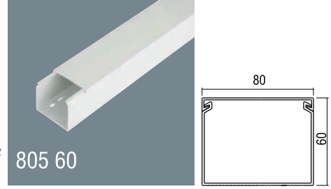
80x60 PVC Kablo Kanalı Kapaklı Satılır Ambalaj: 24m / 12 Boy 80x60 PVC Cable Trunking Complete with cover Packaging: 24m / 12 Pcs
