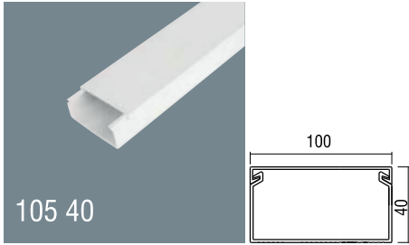
100x40 PVC Kablo Kanalı Kapaklı Satılır Ambalaj: 20m / 10 Boy 100x40 PVC Cable Trunking Complete with cover Packaging: 20m / 10 Pcs
